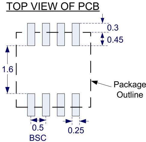
Fig. 20: LGA package land pattern [top view].
