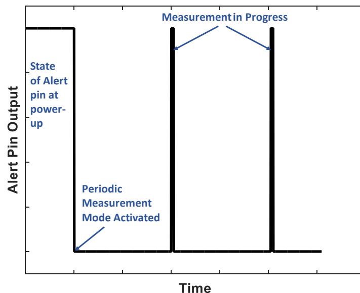
Fig. 12: Alert Pin Functionality – Measurement Active Indicator.
