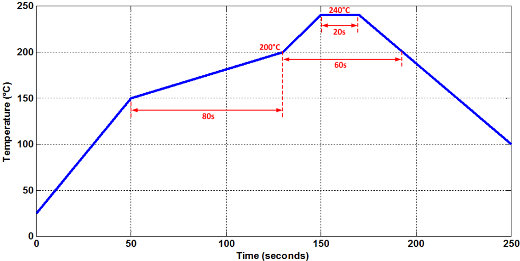
Fig. 22: Recommended lead-free soldering profile
