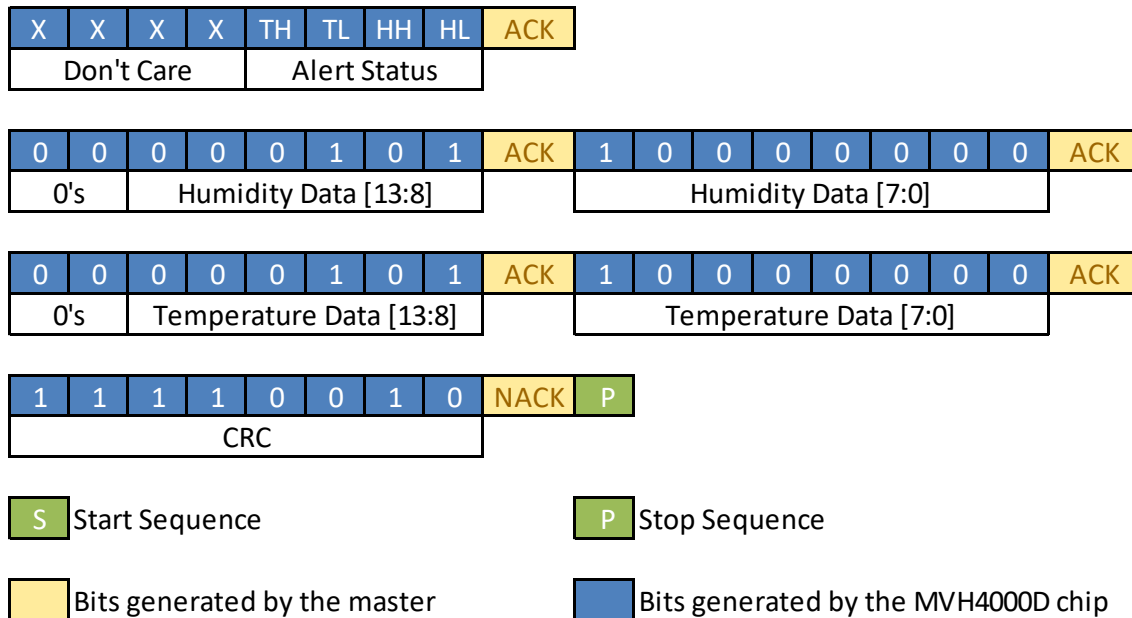
Fig. 14: Data returned from MVH4000D chip when the Alert feature is enabled in Periodic Measurement Mode.
