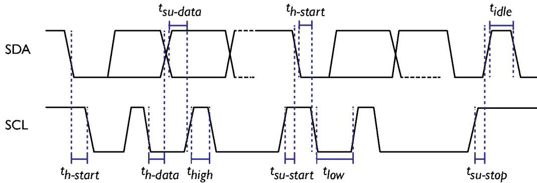
Fig. 18: I 2 C timing diagram.
