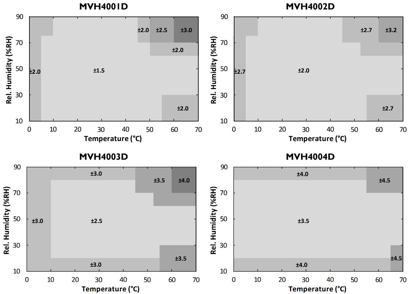
Fig. 5: Relative humidity tolerances across temperature.
