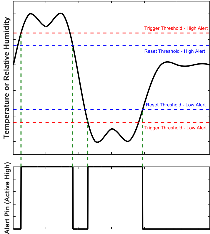
Fig. 13: Example of Alert Pin Functionality in Humidity / Temperature Detection Mode.
