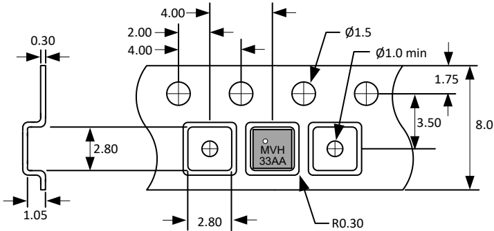
Fig. 21: Packaging tape drawing.
