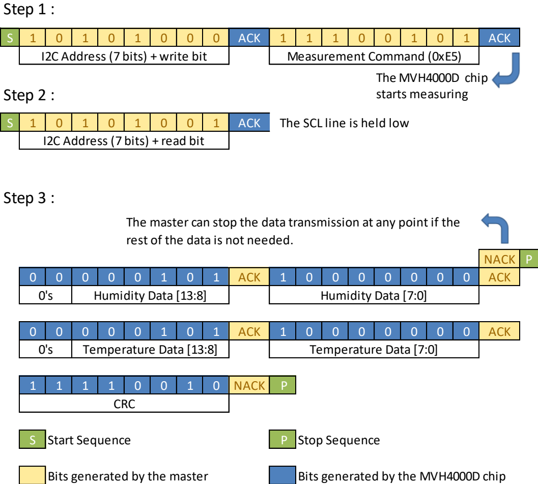
Fig. 8: Typical hold measurement sequence for a humidity and temperature command.
