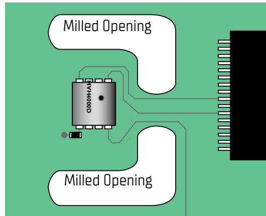
Fig. 23: Thermal isolation of sensor using milled PCB openings.
