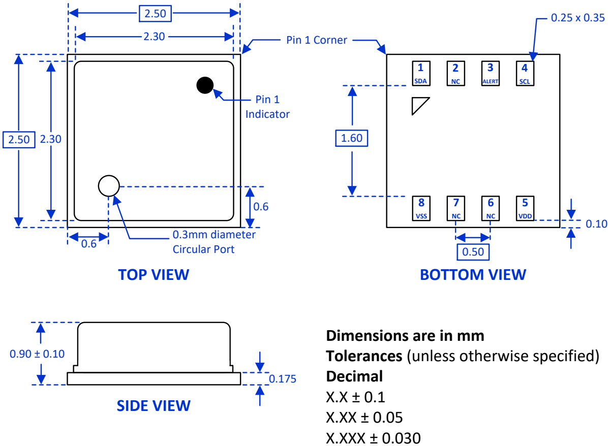
Fig. 19: LGA package drawing.
